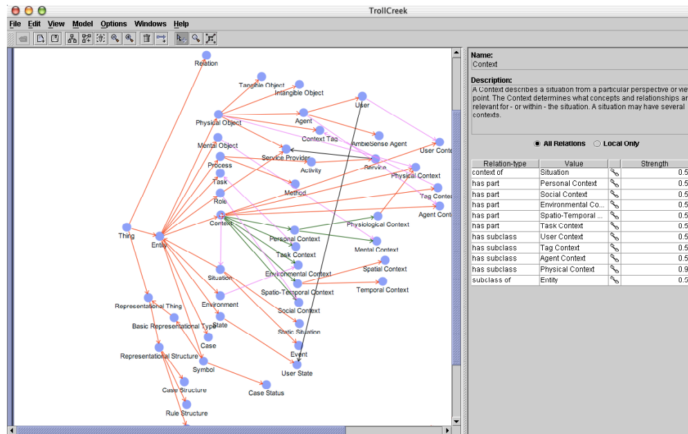
Fig. 4. The TrollCreek Knowledge Modeling Editor
