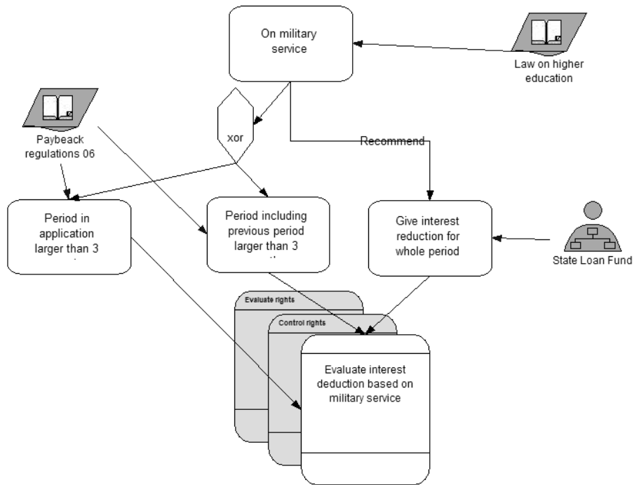
Fig. 3. Implementation of rules, linked to the process model and resource model
